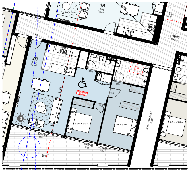
3 PRE ADAPTABLE & LIVABLE UNIT - LEVEL 4 SCALE 1:200 UNITS: 4.02 TOTAL: 1
