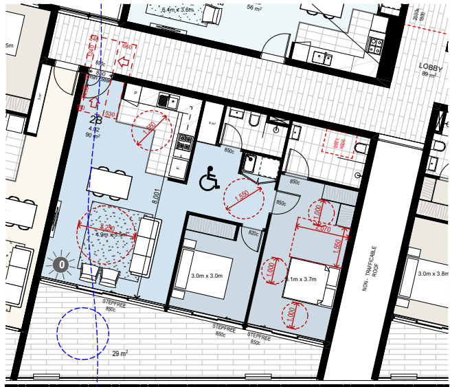
4 POST ADAPTABLE & LIVABLE UNIT - LEVEL 4 SCALE 1:200 UNITS: 4.02 TOTAL: 1
